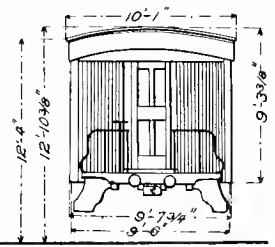
Fig. 88. End Elevation.
